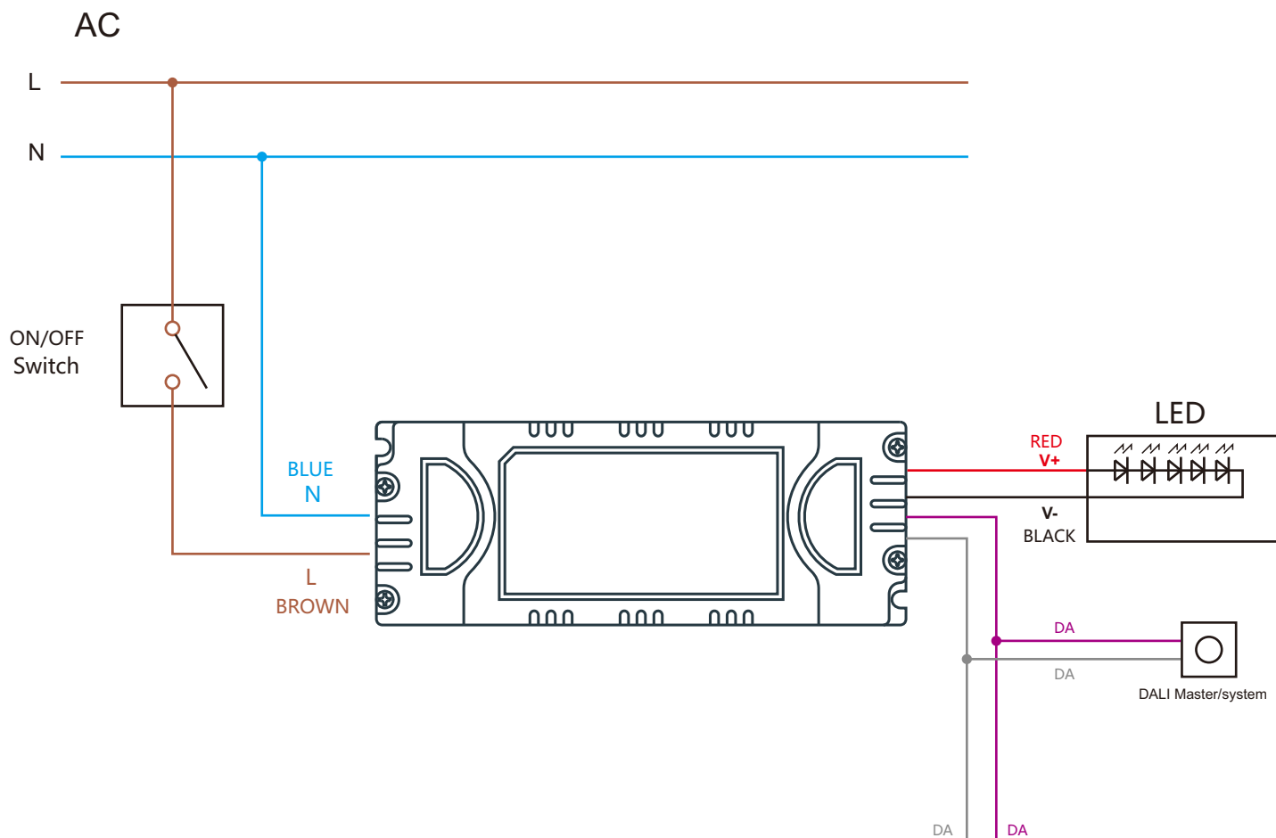
DALI dimmer wiring diagram
