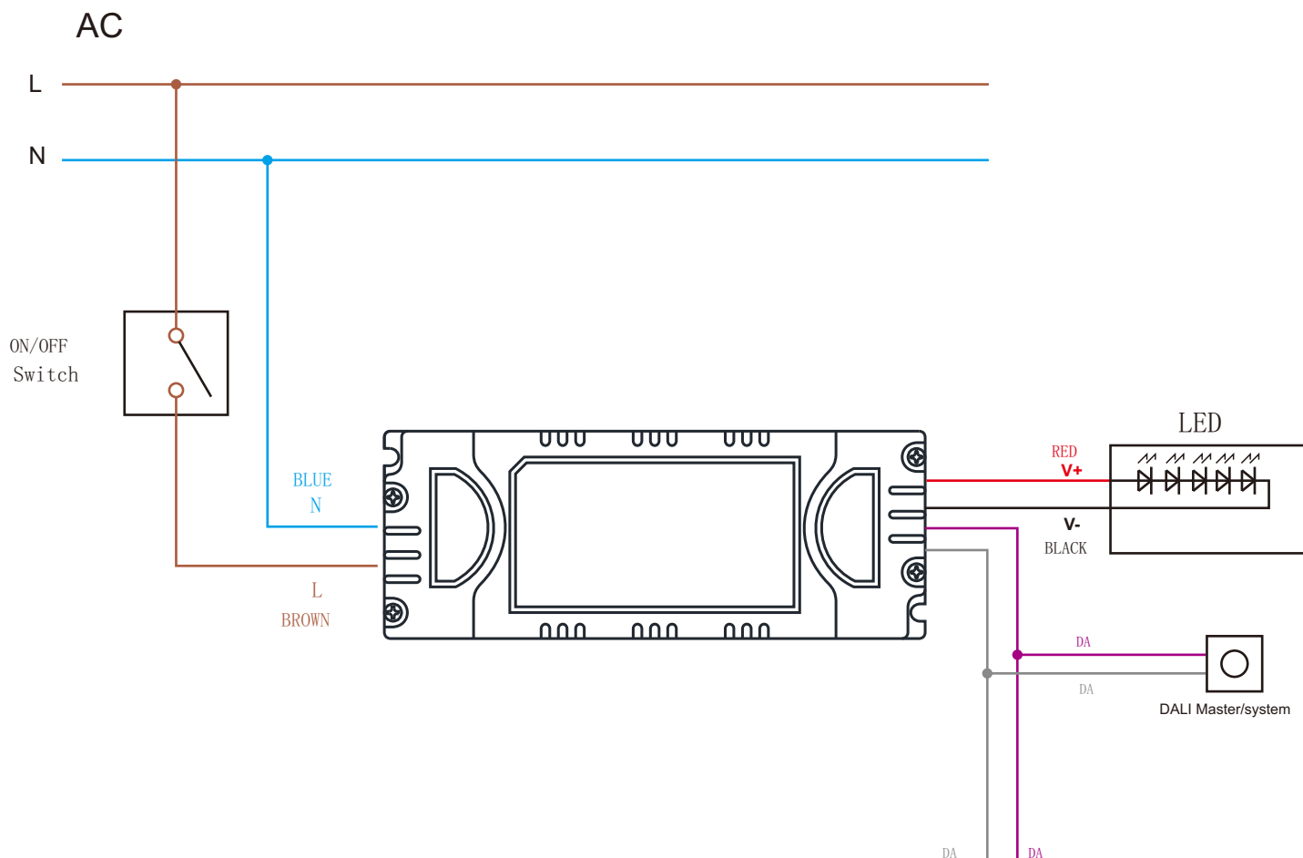
DALI dimmer wiring diagram
